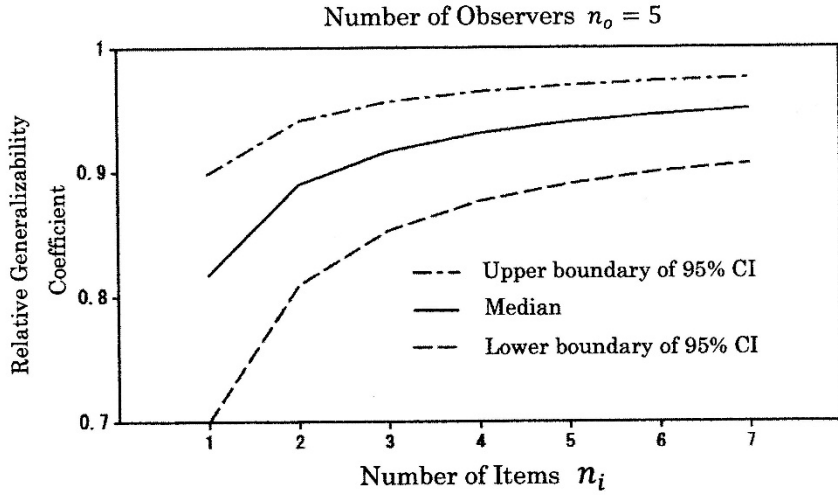
Figure 2. 95% central intervals (CIs) of relative generalizability coefficients for various n_i s with n_o = 5 .
