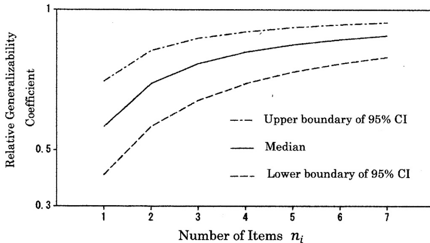
Figure 1. 95% central intervals (CIs) of relative generalizability coefficients for various n_i s.
